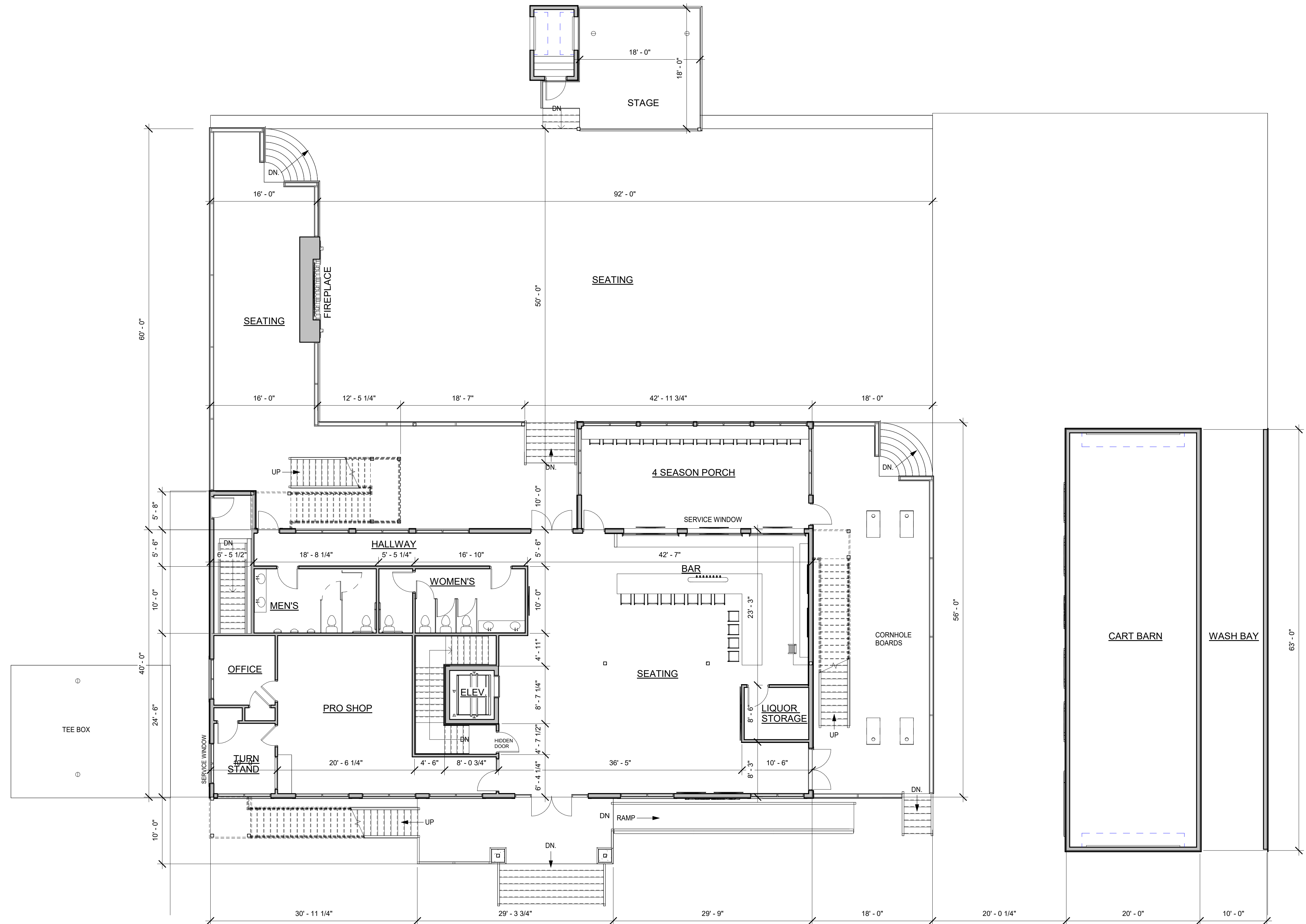
1 MAIN LEVEL FLOOR PLAN A1.1 1/8" = 1'-0"
