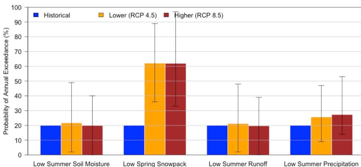
Figure 20. Projected Future Drought in Morrow County
