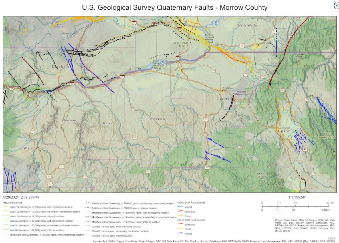
Figure 23. USGS Quaternary Faults in Morrow County
