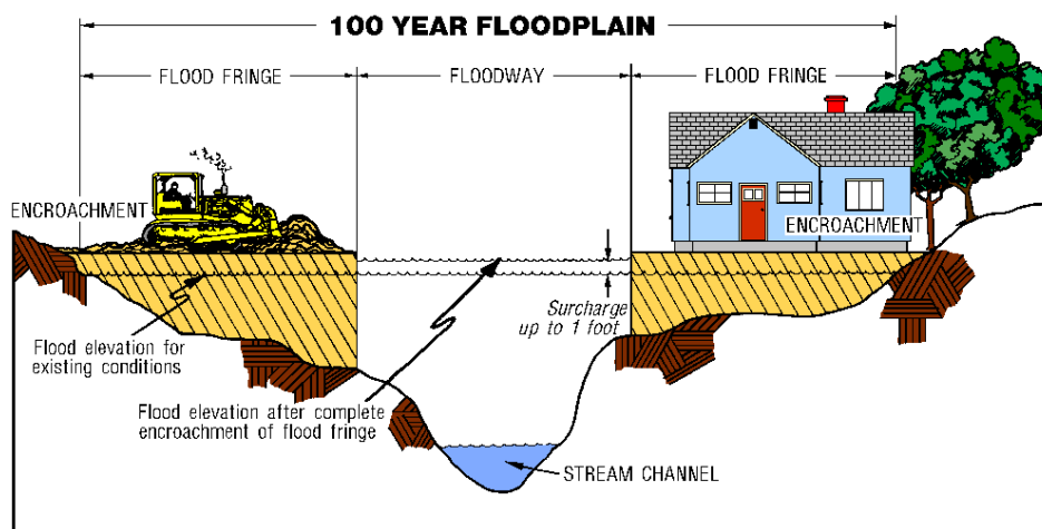
Figure 30. Floodplain Schematic
