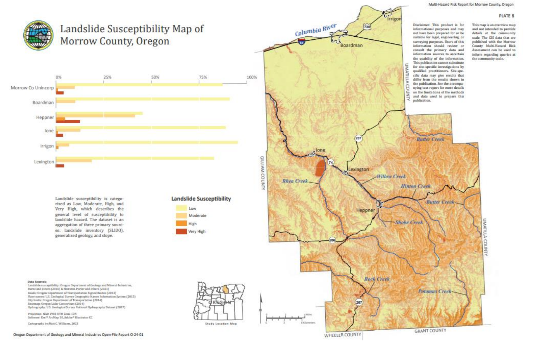
Figure 31. Landslide Susceptibility Map of Morrow County, Oregon
