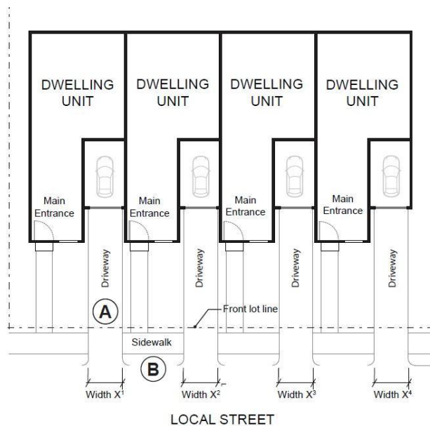
Figure 3.2.5.a. Driveway Approach Width and Separation on Local Street
