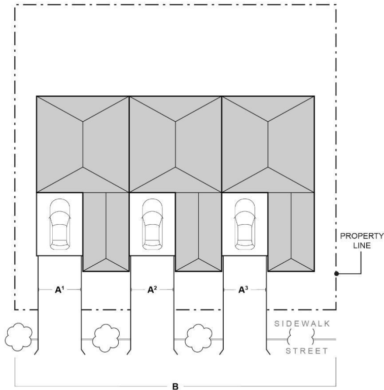
Figure 3.2.4.a. Width of Garages and Parking Areas
