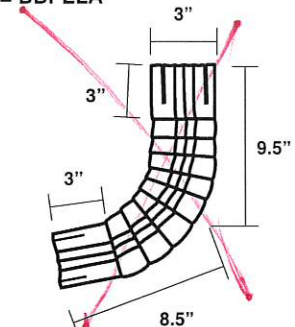
3" x 4" Downspout Elbow A-Style 26 Ga. = BBPELA
