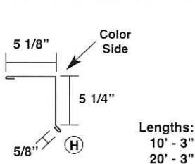
Alternate Rake Trim MDAR
