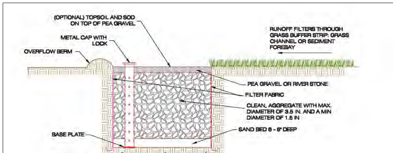
Figure 4.17. Example design of an infiltration trench.
