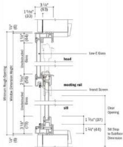
Vertical Section Arch Single-Hung
