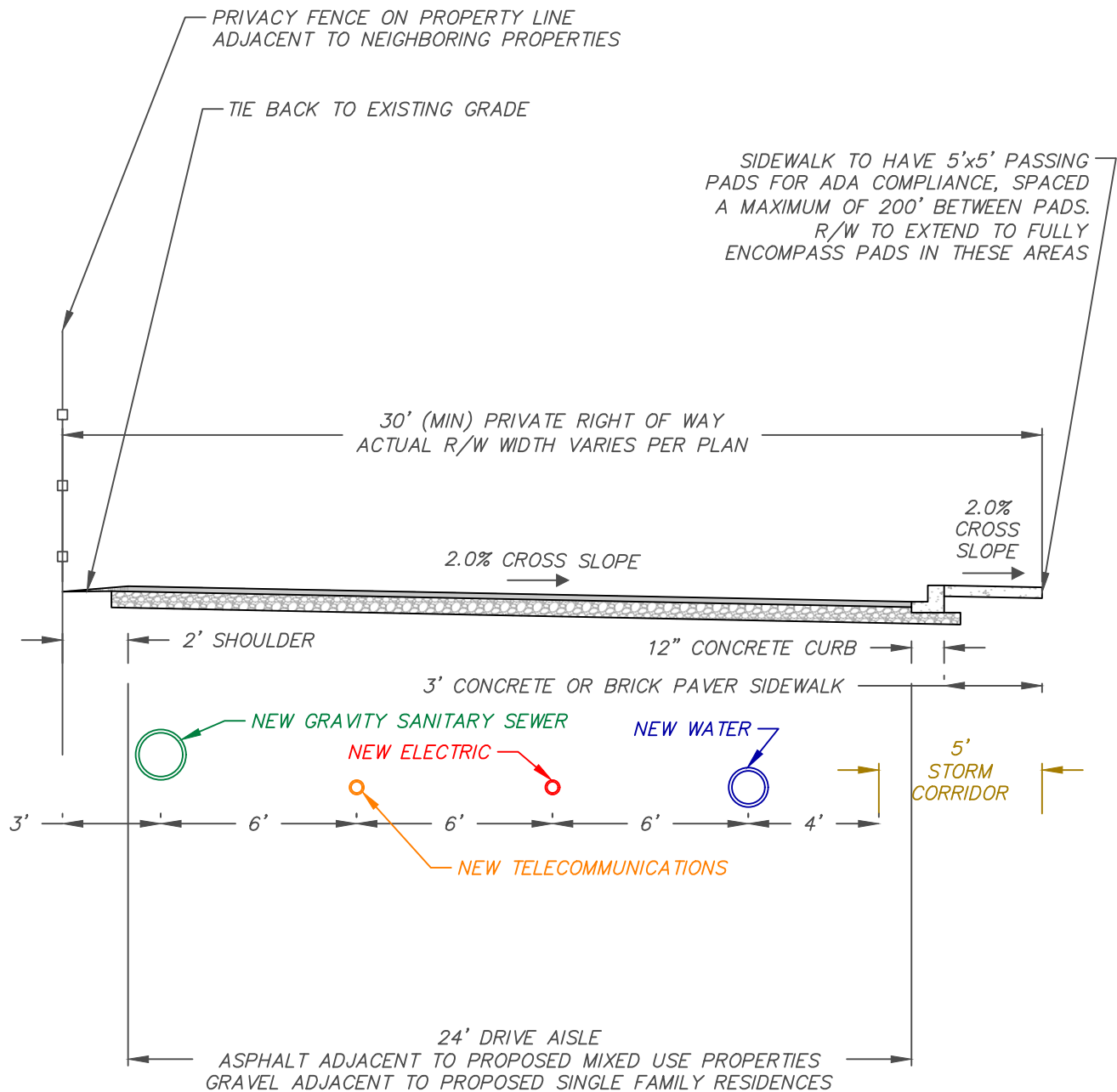
30' RIGHT-OF-WAY/EASEMENT DETAIL N.T.S.
