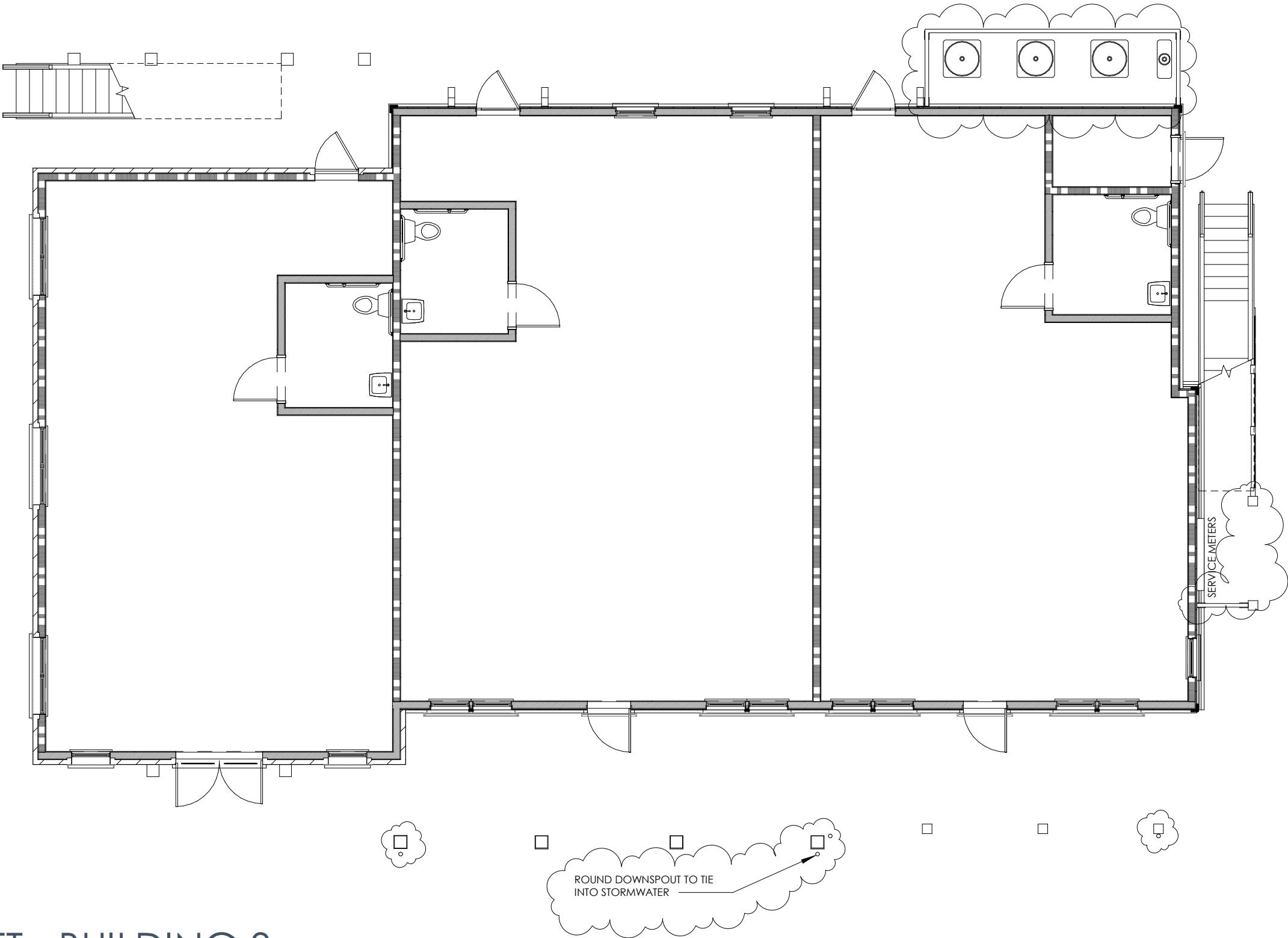
① FIRST FLOOR PLAN 1/8" = 1'-0"
