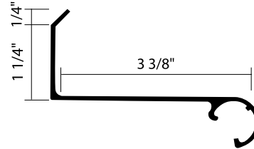
3 - 3/8" Female Hinge
