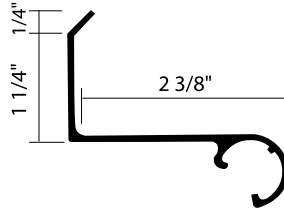
2 - 3/8" Female Hinge
