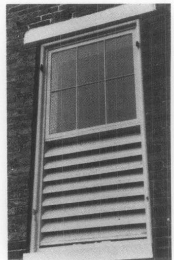
Figure 18. Heavy duty wooden slatted louvers were custom fabricated to replace the deteriorated lower sash. The upper sash were rebuilt to retain the historic appearance and to allow light into this vacant historic building. Refer back to Fig. 1 for a view of the building. Photo: Charles E. Fisher, NPS. Drawing by Thomas Vitanza.
