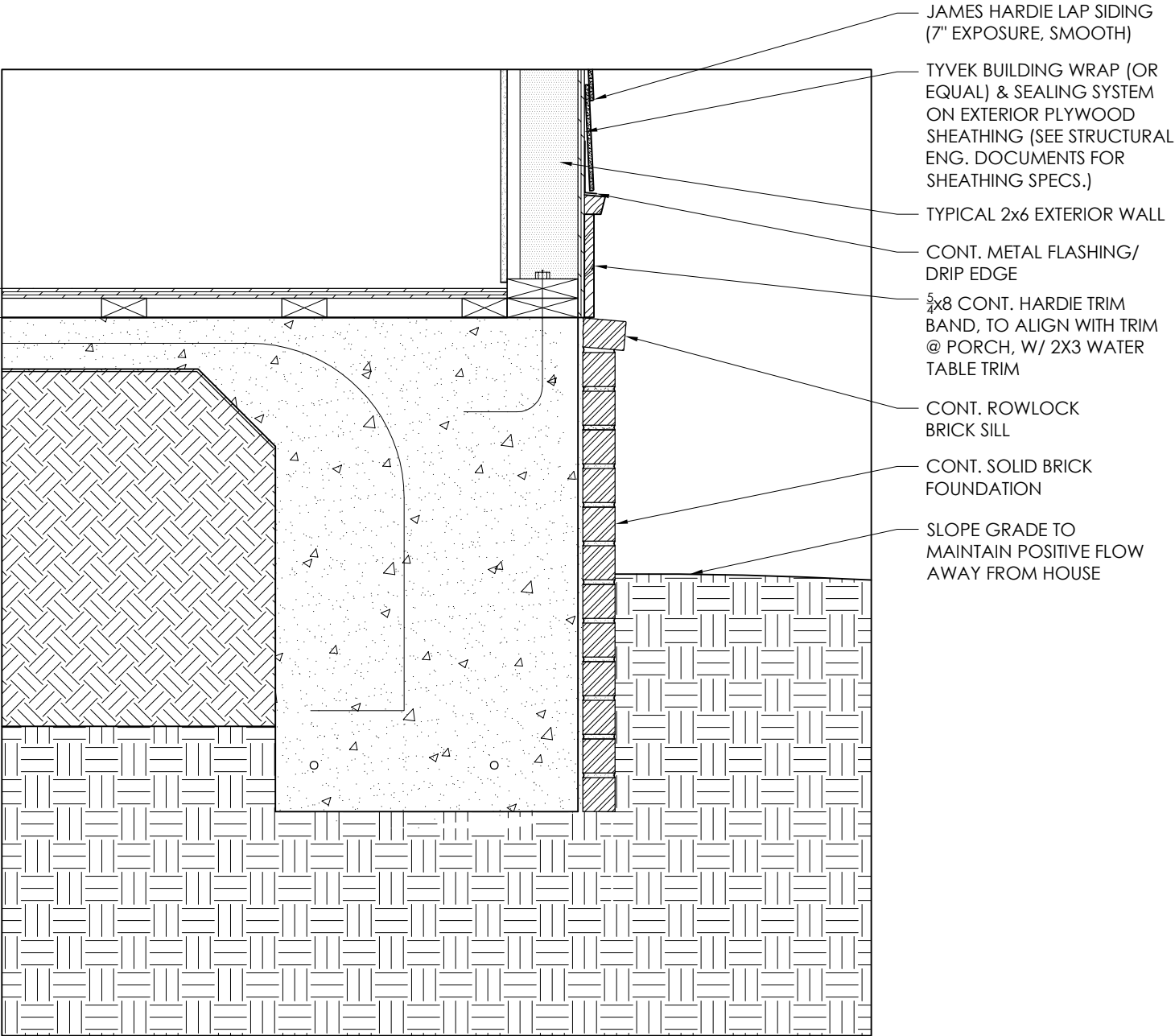
TYP. MAIN HOUSE FDTN. - REVISED
