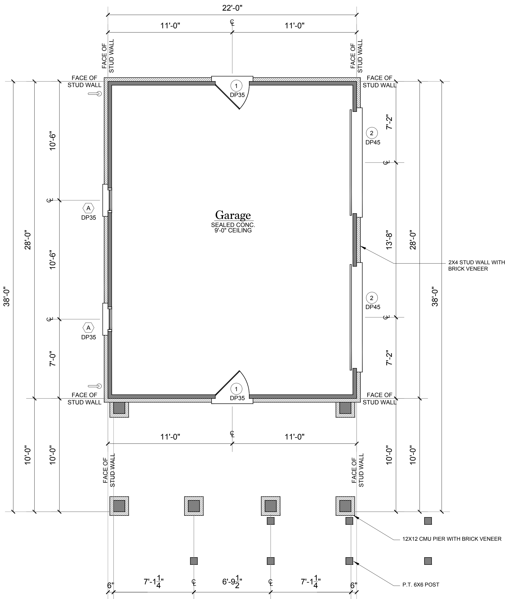
A GROUND FLOOR PLAN A2 SCALE: 1/4"=1'-0"
