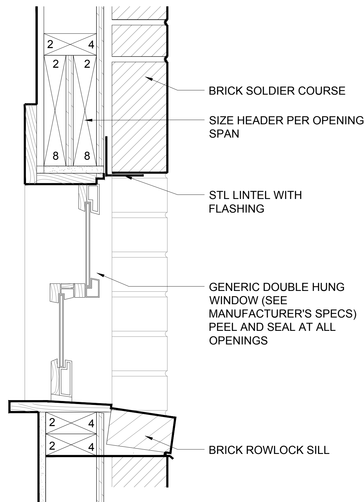
C WINDOW DETAIL @ BRICK A2 SCALE: 3/8"=1'-0"
