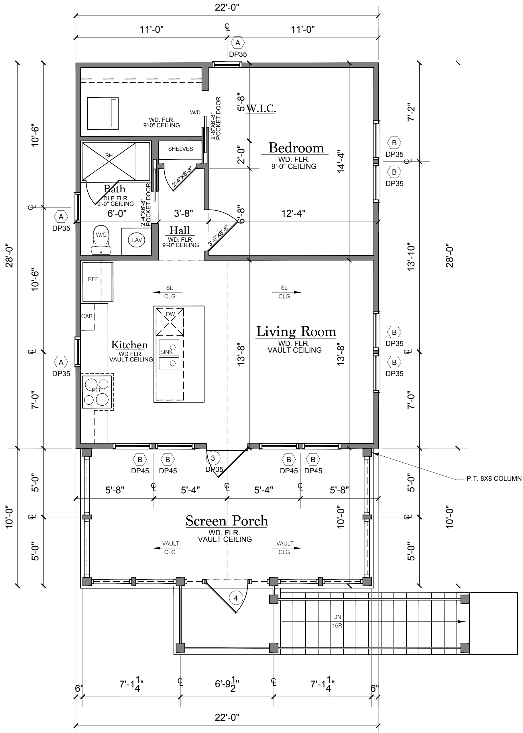
B FIRST FLOOR PLAN A2 SCALE: 1/4"=1'-0"
