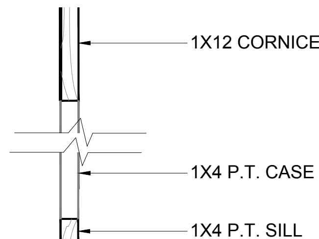
D WINDOW TRIM DETAIL @ SIDING A2 SCALE: 3/8"=1'-0"
