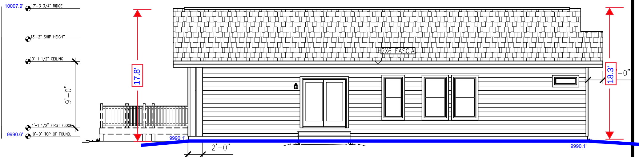
REAR
