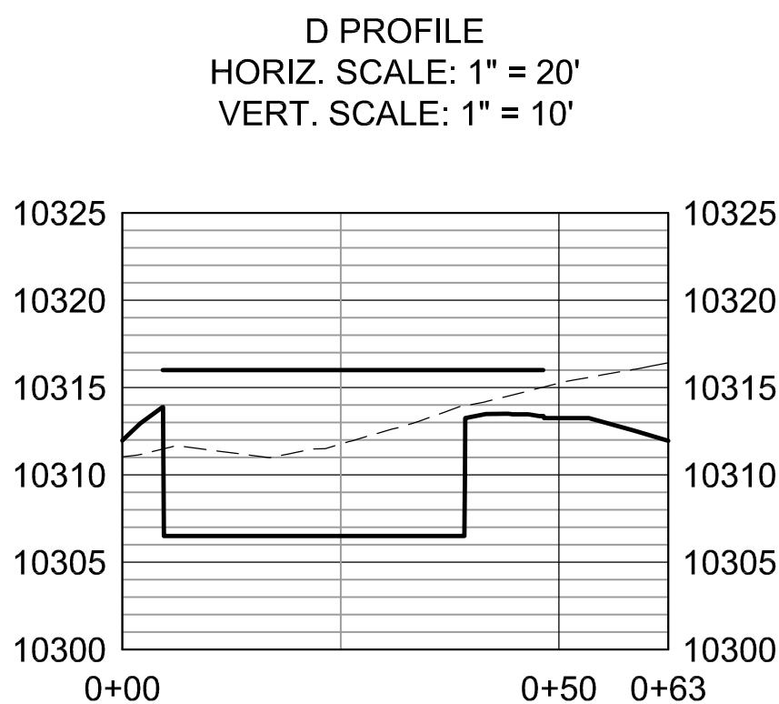
4 GRADING SECTION D-D C2.1 NO SCALE
