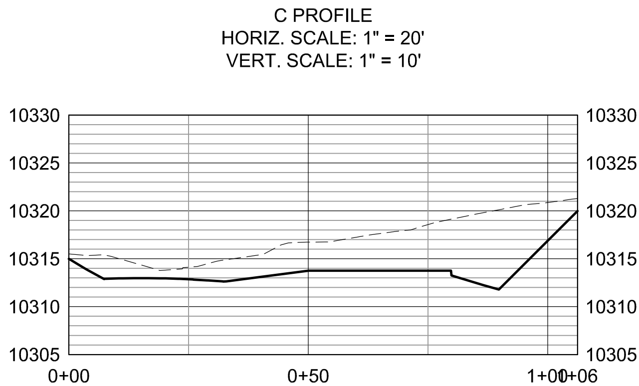
3 GRADING SECTION C-C C2.1 NO SCALE
