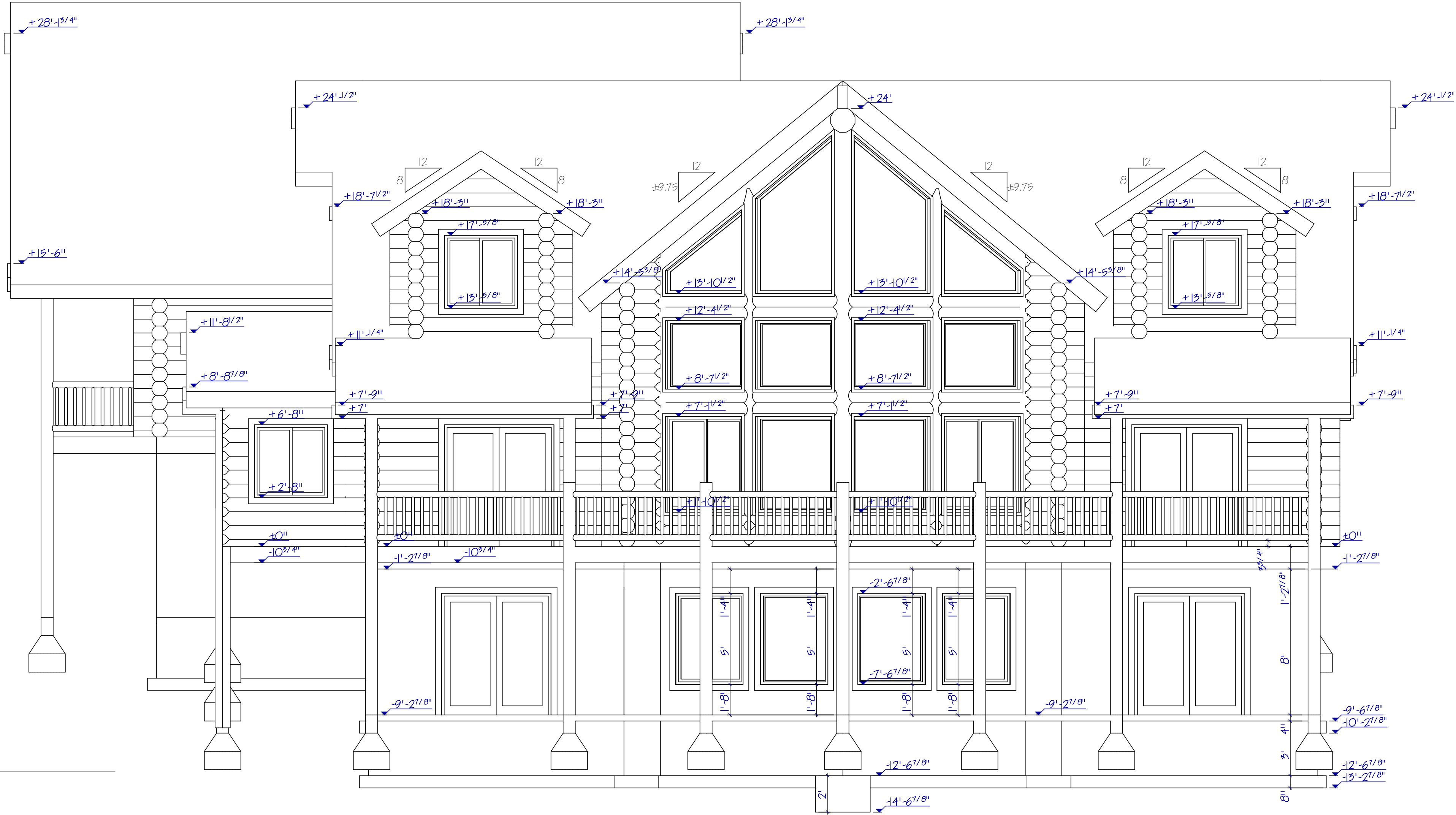
Front Elevation
