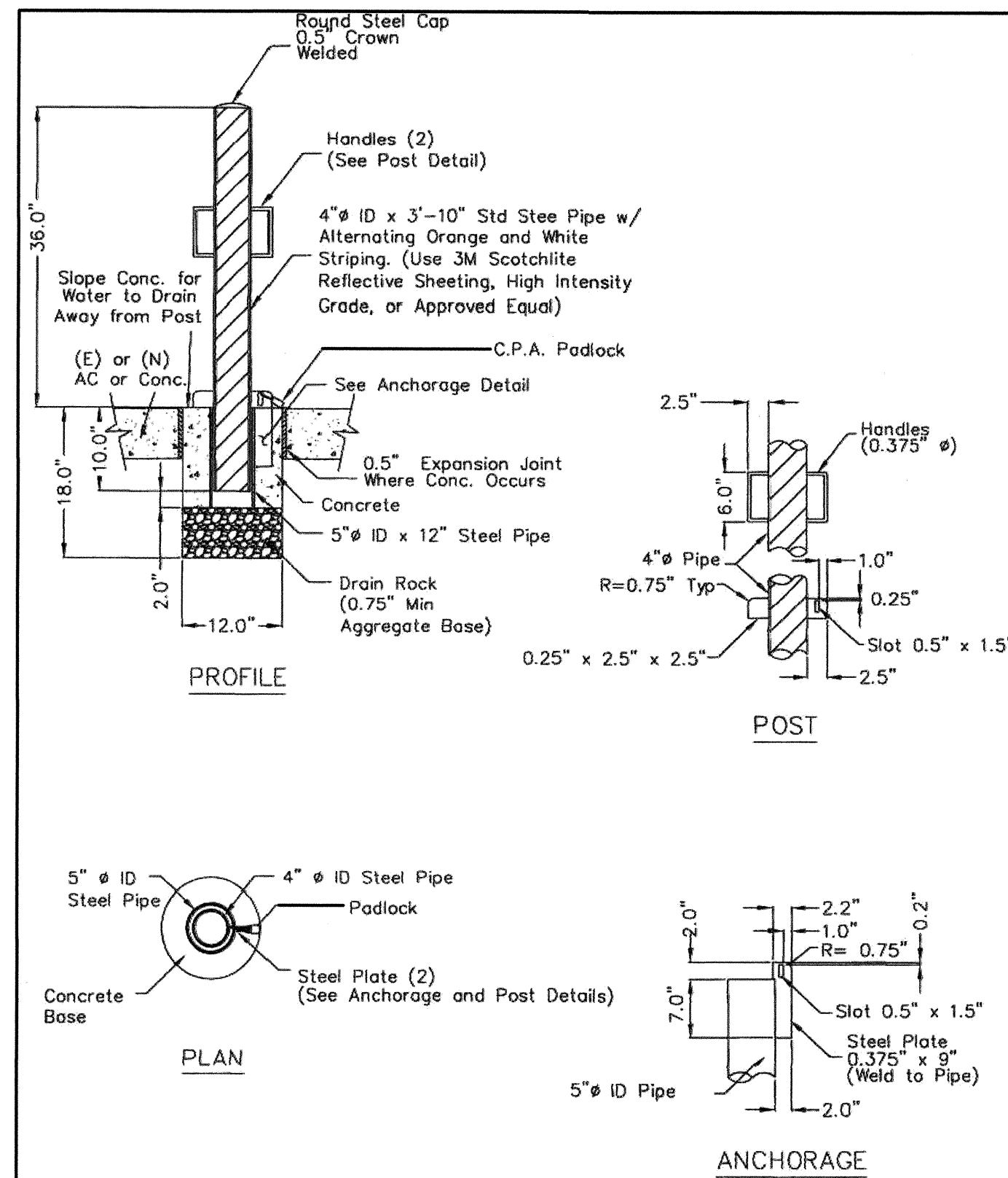
6 REMOVABLE BOLLARD DETAIL NO SCALE
