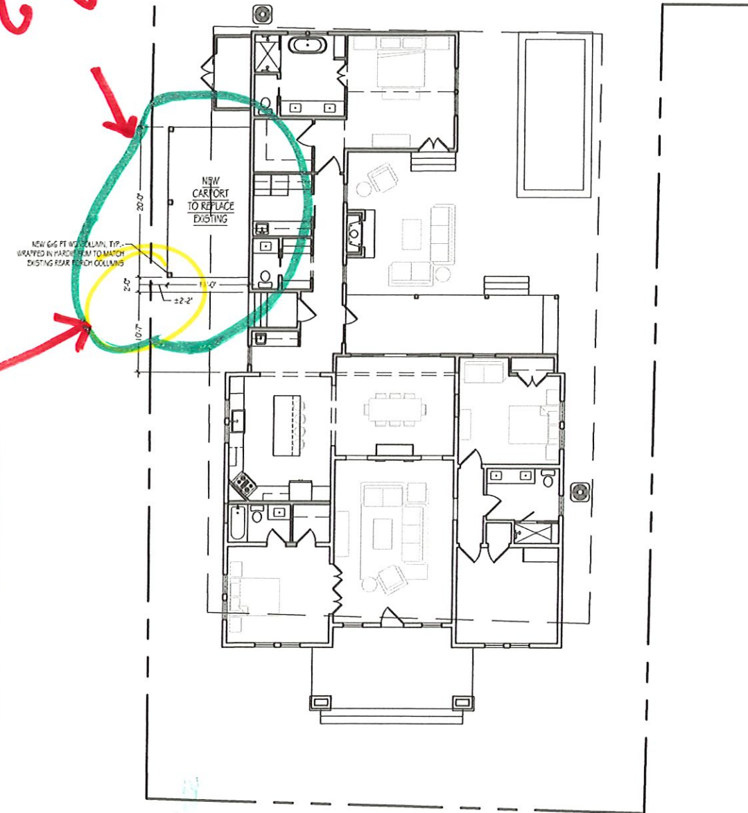
2 SITE PLAN Scale: 3/32" = 1'-0"
