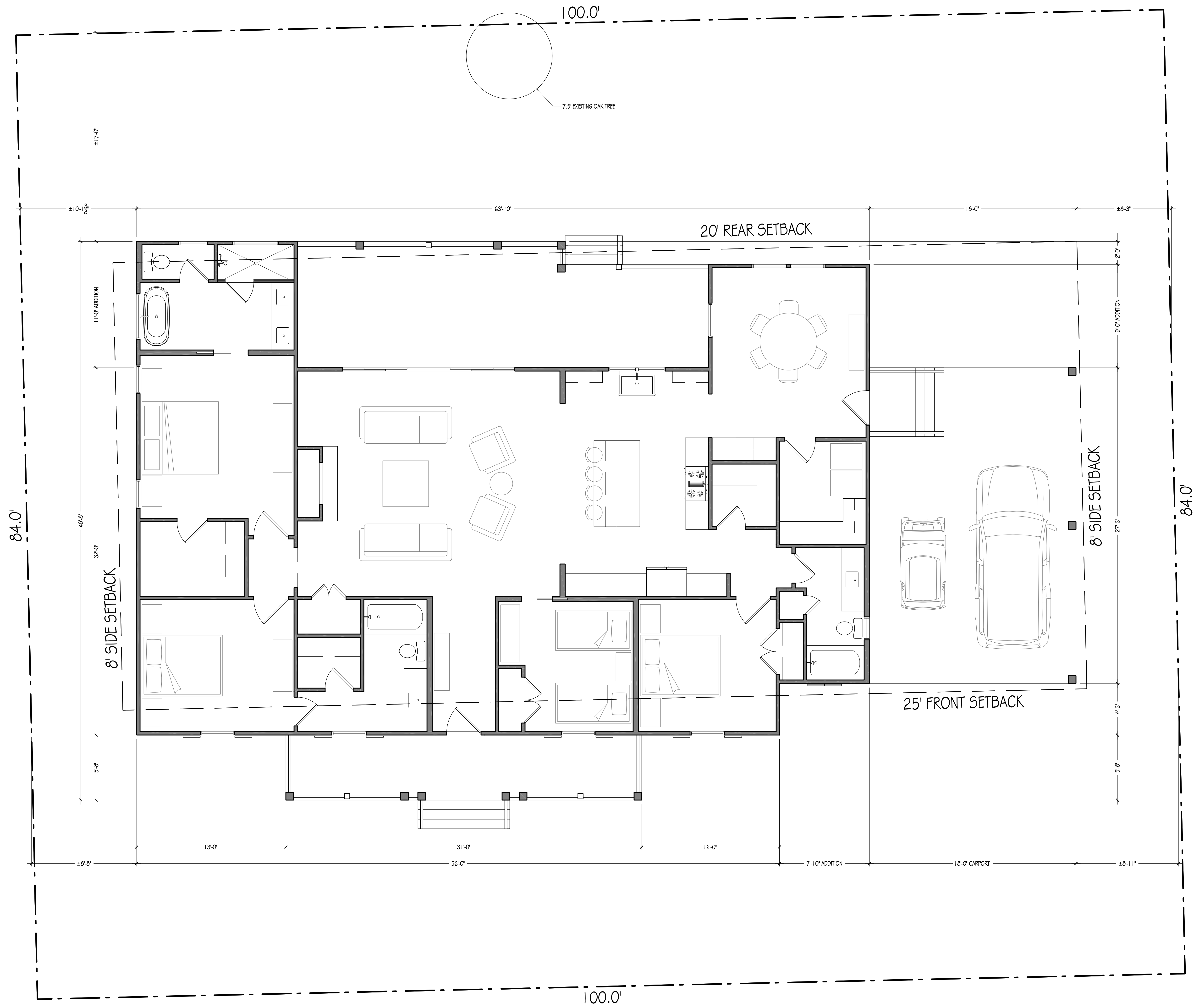
1 PROPOSED SITE PLAN Scale: 1/4"=1'-0"
