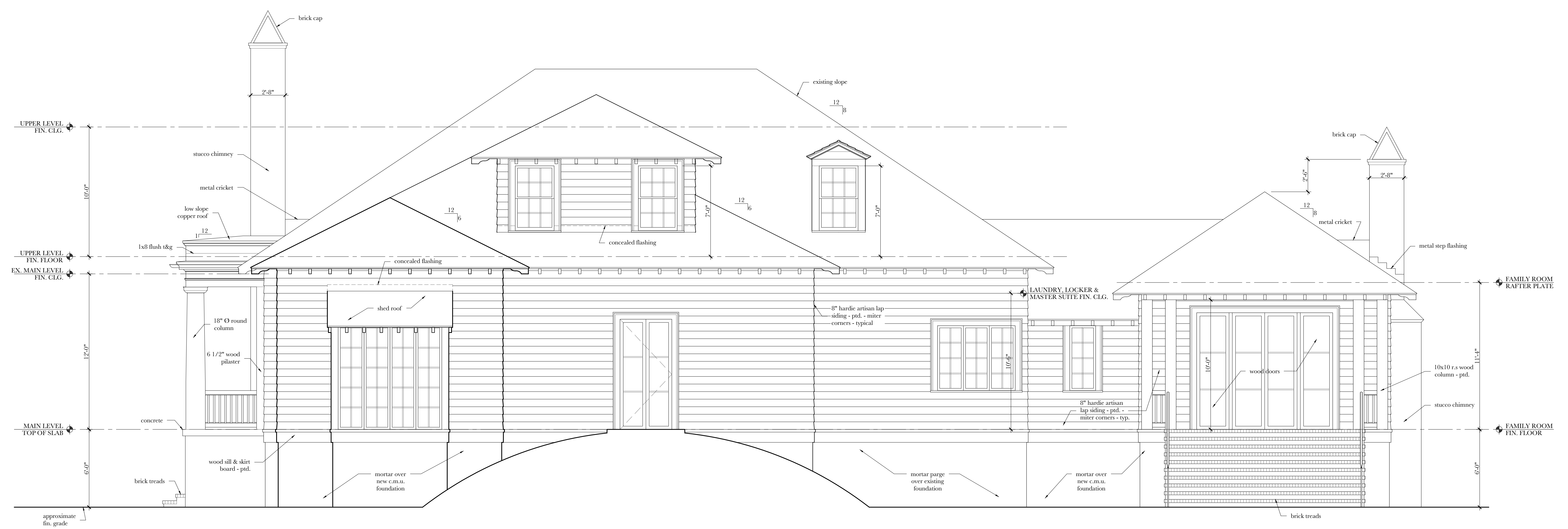
1 rear elevation
