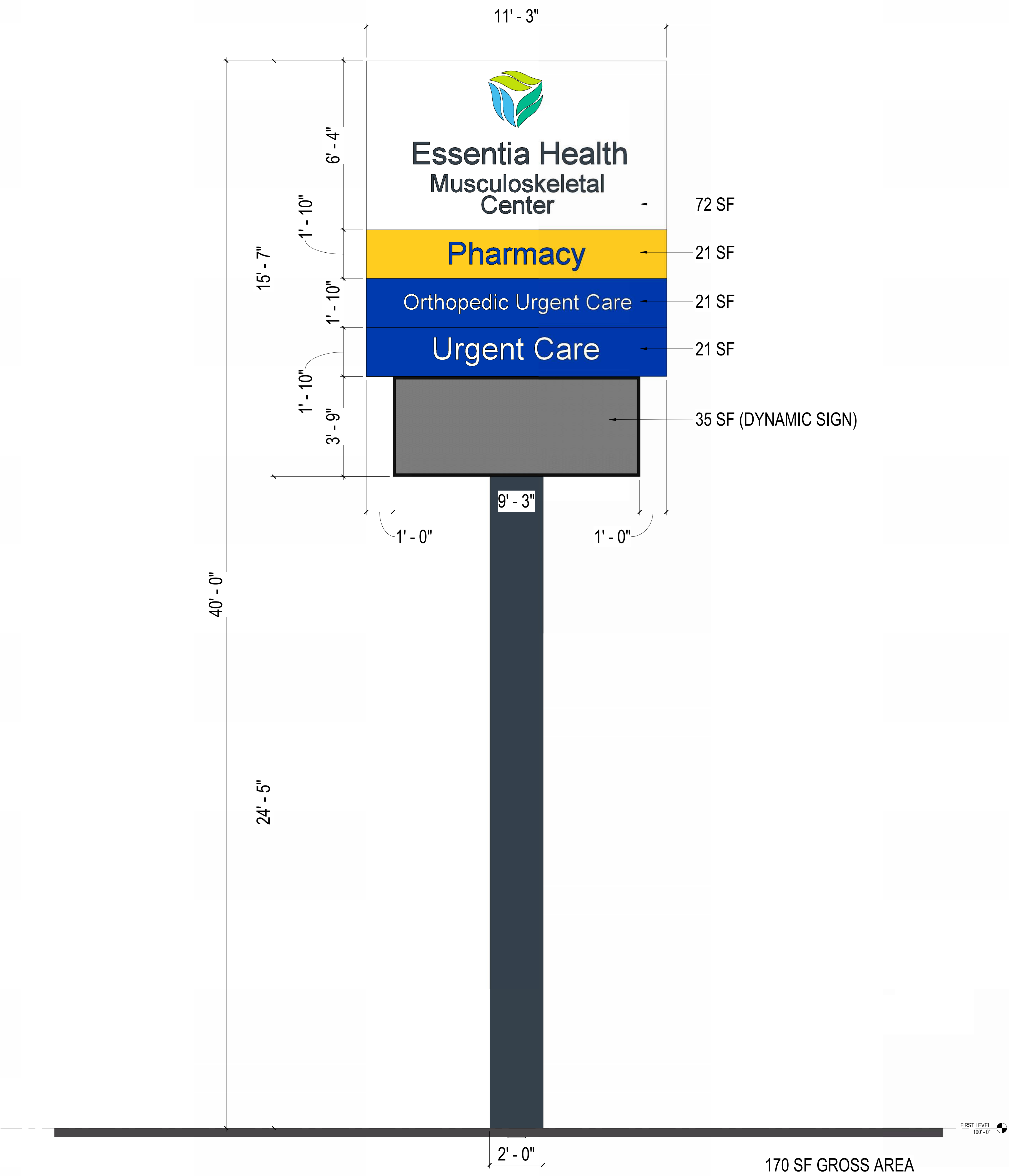
1 ELEVATION 1/2" = 1'-0"
