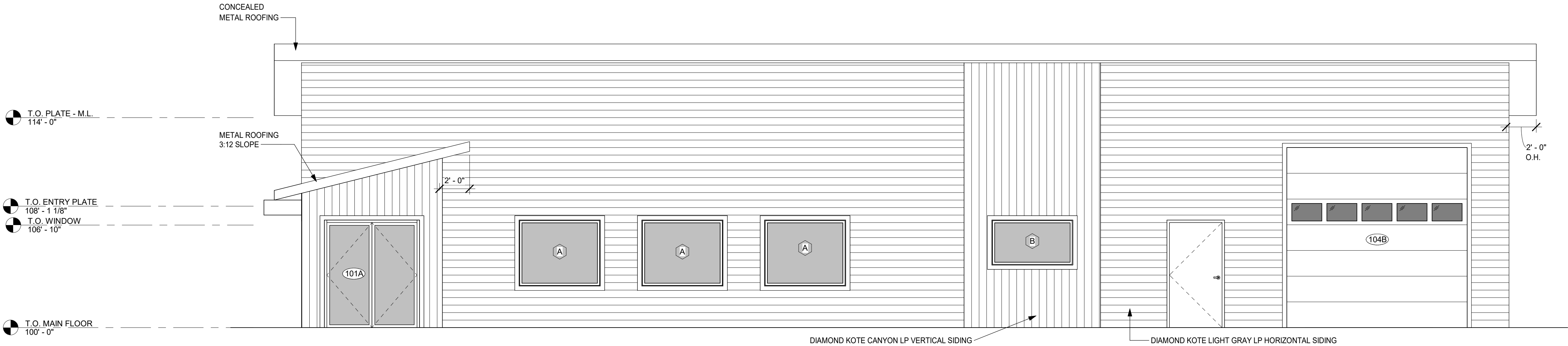
1 SOUTH ELEVATION A2.2 1/4" = 1'-0"
