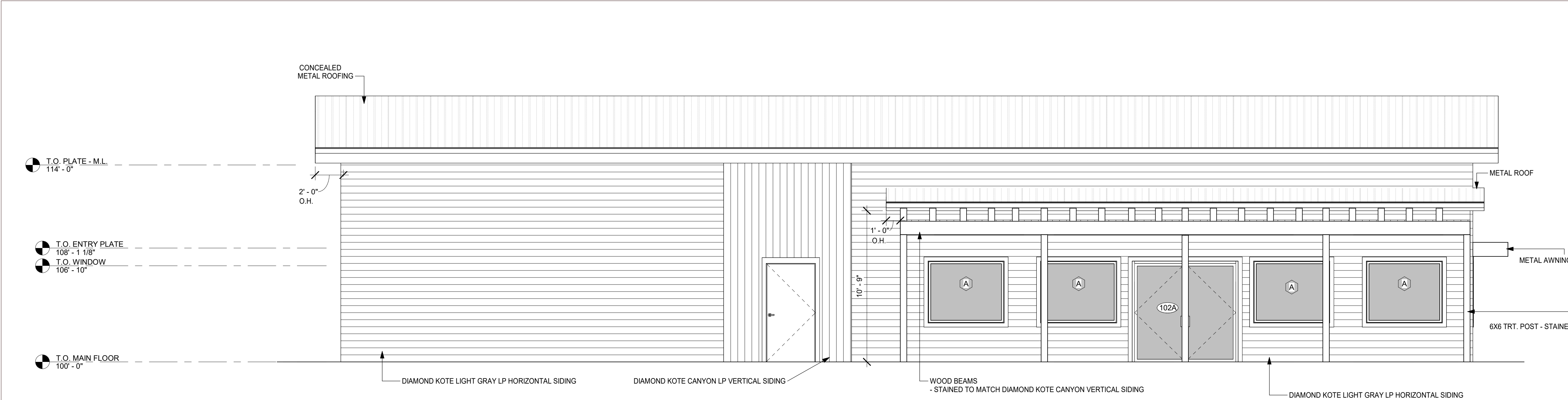
1 NORTH ELEVATION A2.1 1/4" = 1'-0"
