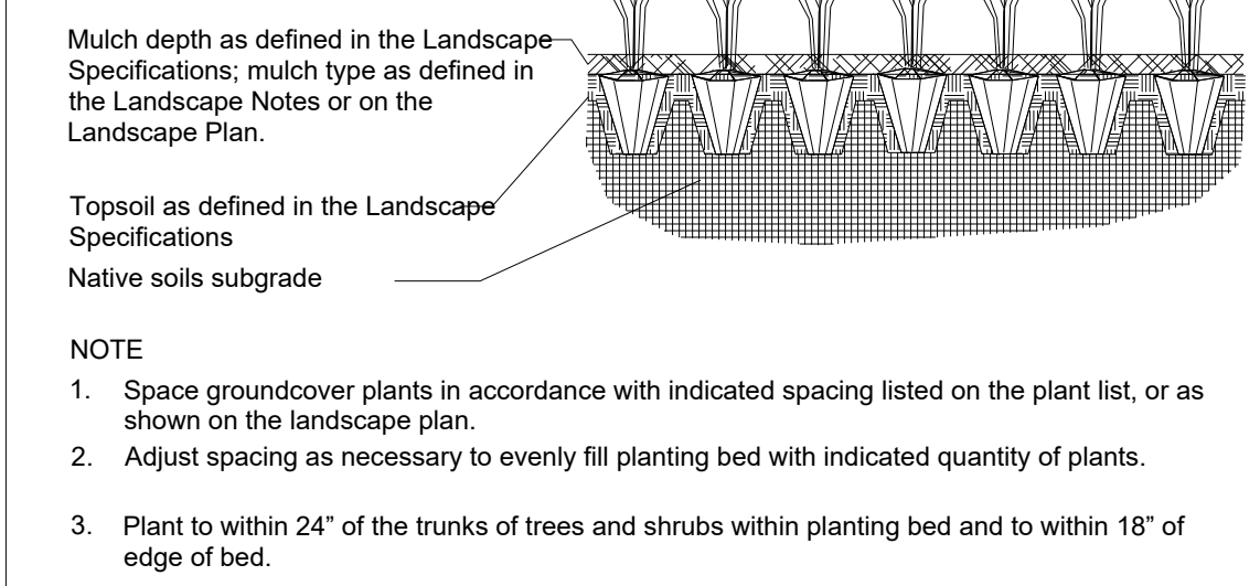
3 GROUND COVER PLANTING DETAIL SCALE: NTS
