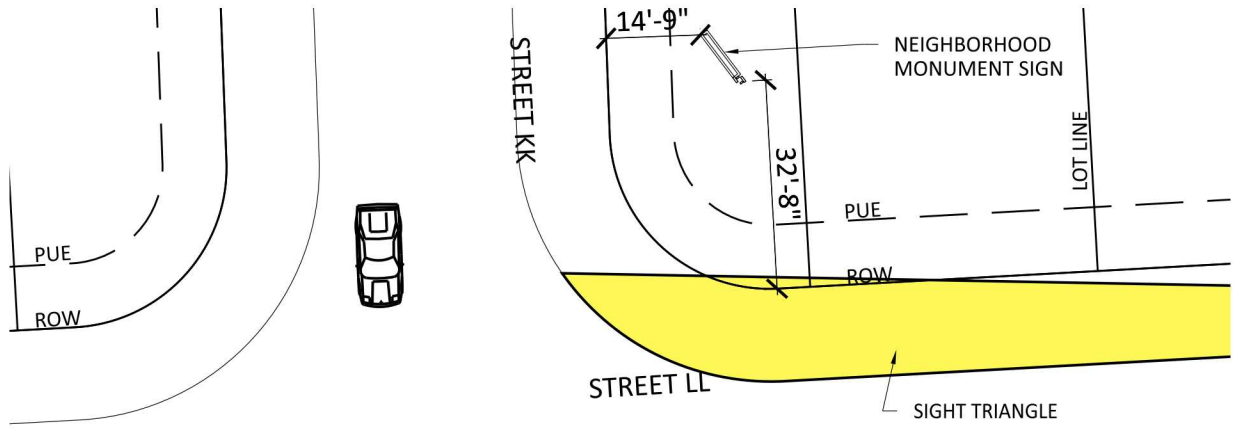
B-12 NEIGHBORHOOD MONUMENT SIGN DETAIL PLAN
