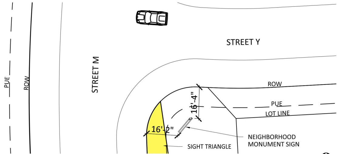
B-9 NEIGHBORHOOD MONUMENT SIGN DETAIL PLAN
