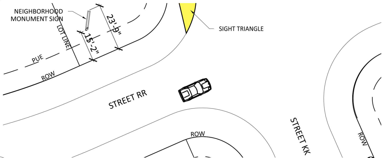
B-13 NEIGHBORHOOD MONUMENT SIGN DETAIL PLAN
