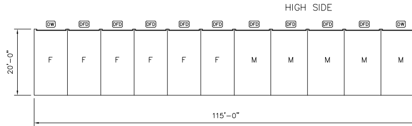
F - 20'-0" x 115'-0" x 8'-4" 1/4:12 PITCH LEAN-TO BUILDING SYSTEM
