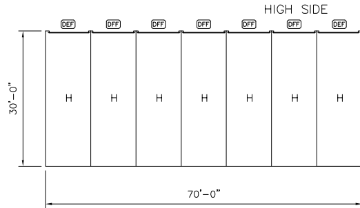
A – 30'-0" x 70'-0" x 8'-4" 1/4:12 PITCH LEAN-TO BUILDING SYSTEM
