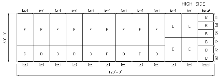
E - 30'-0" x 120'-0" x 8'-4" 1/4:12 PITCH LEAN-TO BUILDING SYSTEM
