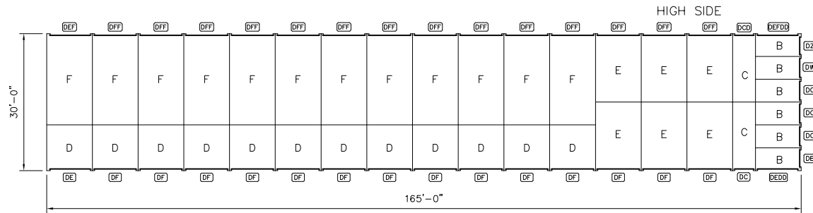
D - 30'-0" x 165'-0" x 8'-4" 1/4:12 PITCH LEAN-TO BUILDING SYSTEM
