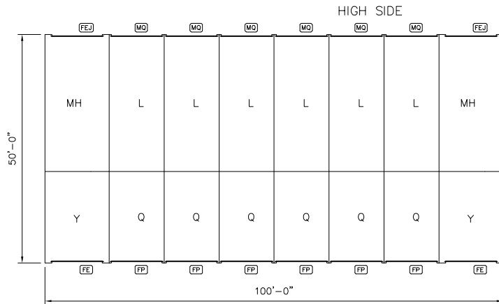
B & C – 50'-0" x 100'-0" x 10'-4" 1/4:12 PITCH LEAN-TO BUILDING SYSTEM
