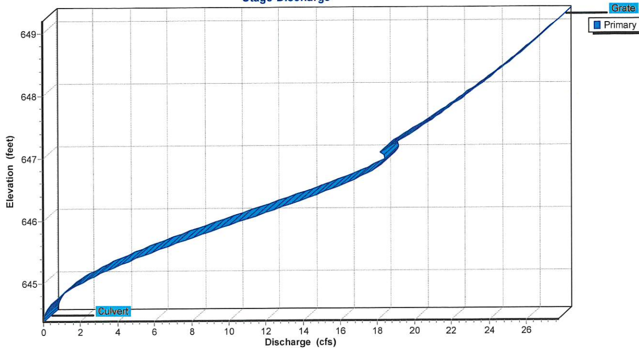
Stage-Discharge
