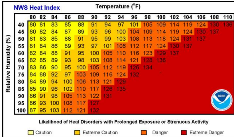
Chart 22: Heat Index
