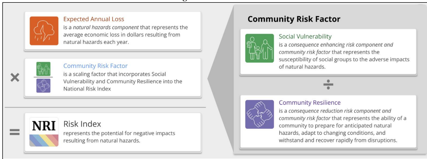
Figure 1: FEMA NRI
