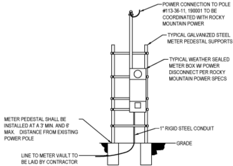
1 METER PEDESTAL FOR RISER CONNECTION SCALE: NONE
