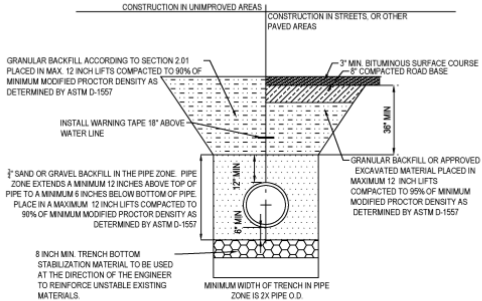
1 TRENCH DETAIL
