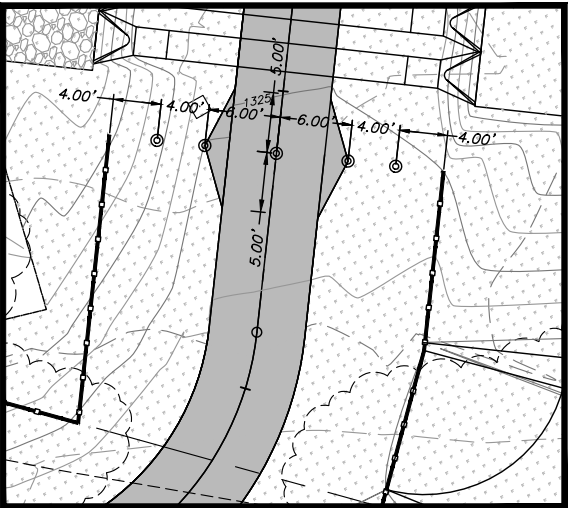
PIPE BOLLARD LAYOUT
