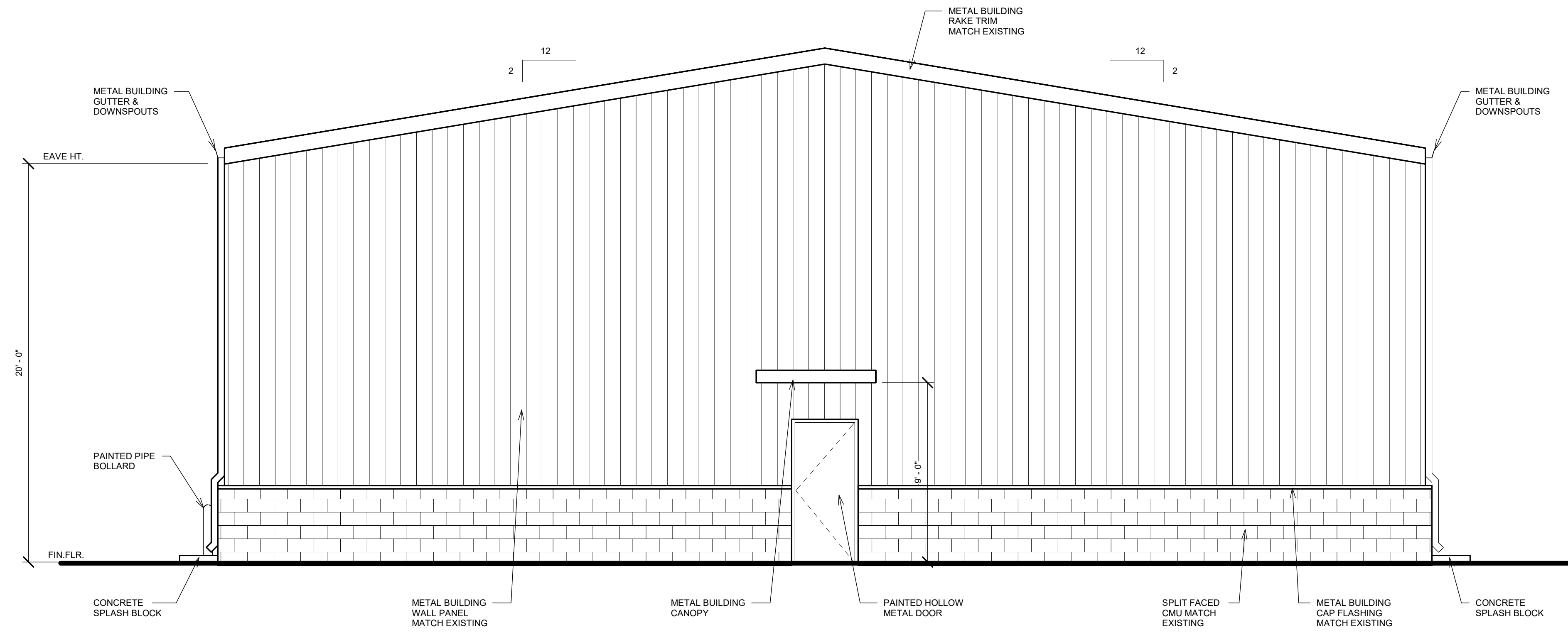
2 EAST ELEVATION 1/4" = 1'-0"
