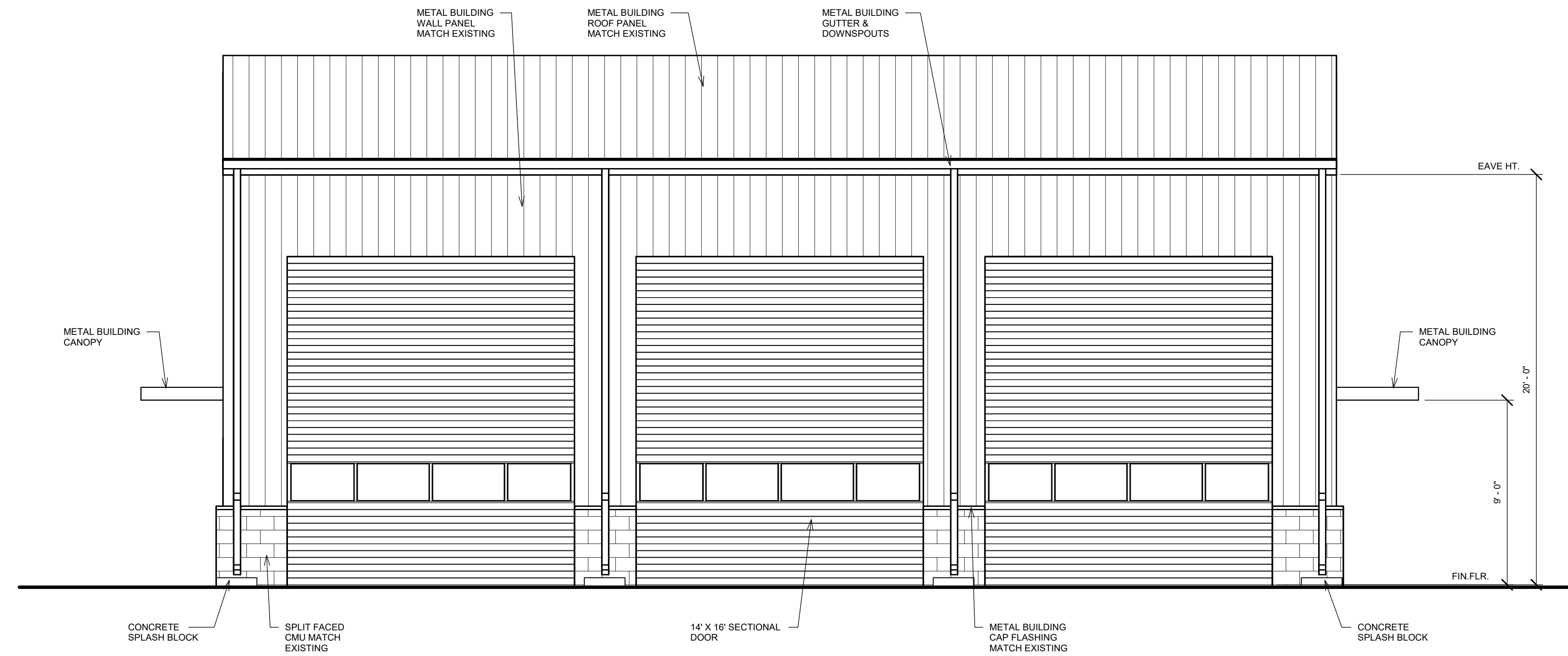
2 NORTH ELEVATION 1/4" = 1'-0"
