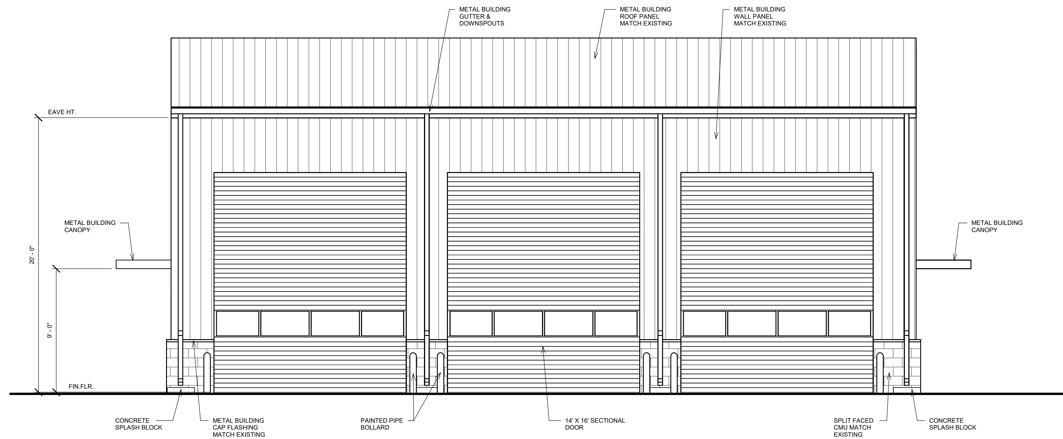
1 SOUTH ELEVATION 1/4" = 1'-0"
