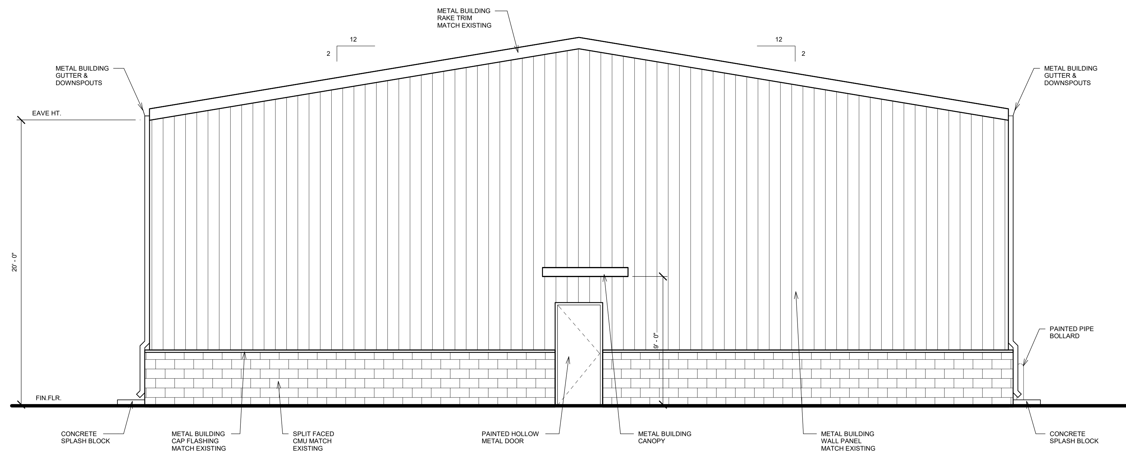
1 WEST ELEVATION 1/4" = 1'-0"
