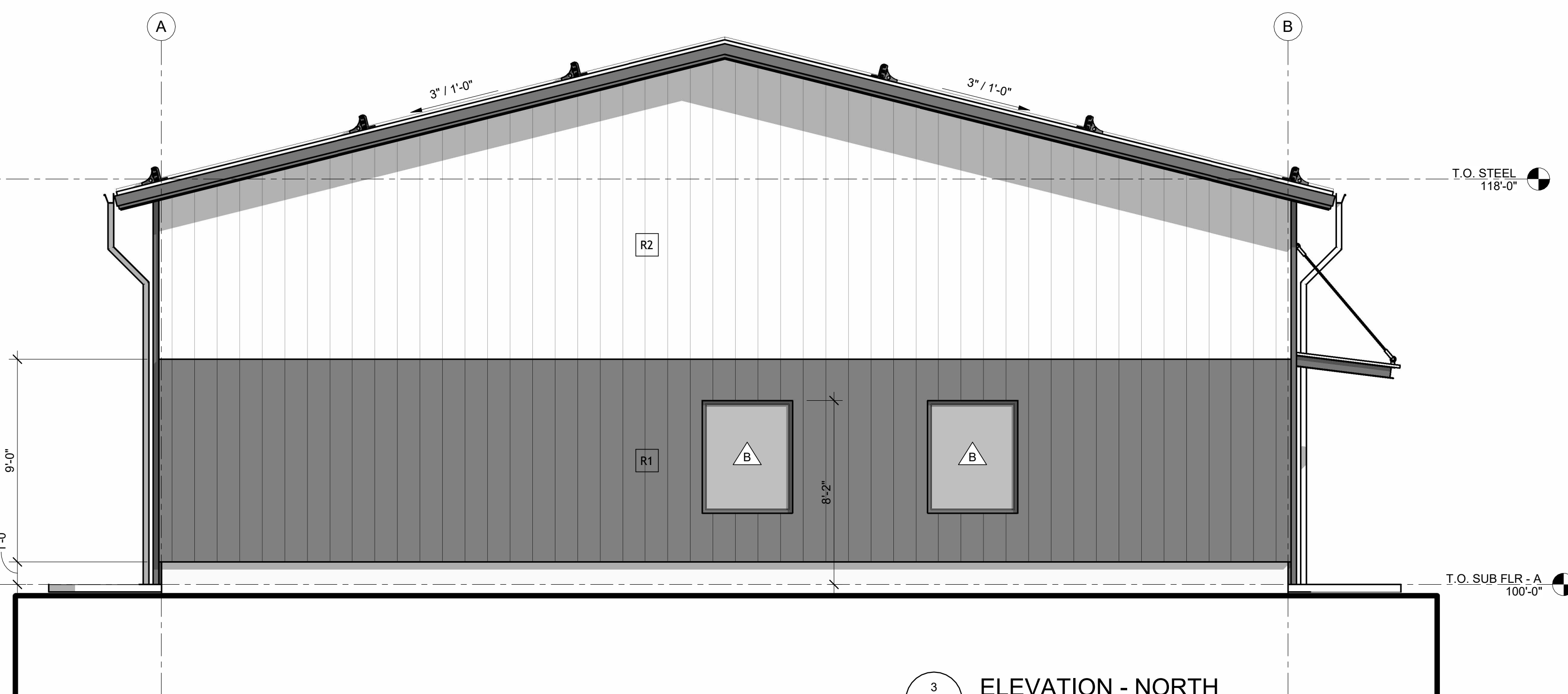
3 ELEVATION - NORTH A201 1/4" = 1'-0"
