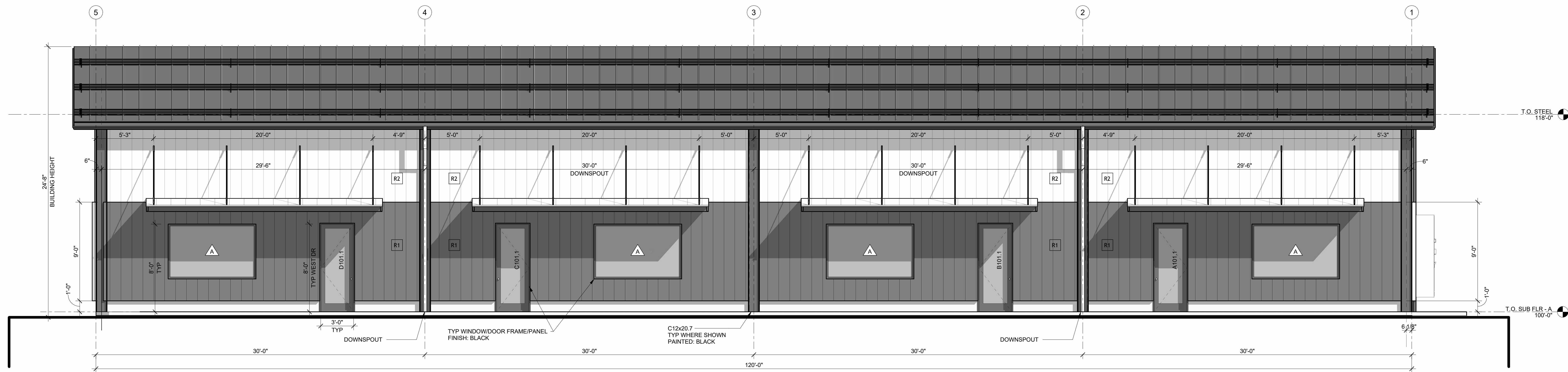
2 ELEVATION - WEST A201 1/4" = 1'-0"
